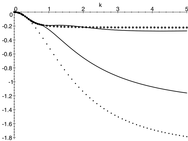
Fig. 7 Attenuation rates with the regularized super-Burnett approximation as the initial condition for the Newton method. Dots: The regularized super-Burnett approximation. Solid: The first and the second Newton iterations. Circles: The exact solution to the invariance equation
