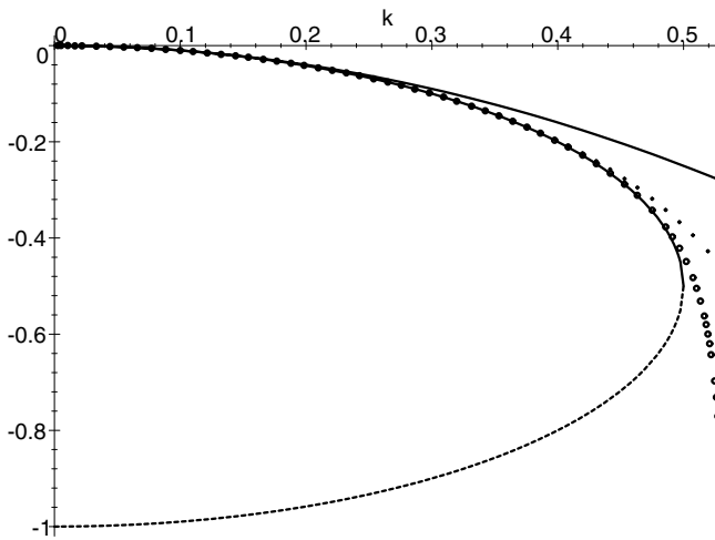
Fig. 8 The diffusion mode with the Euler initial approximation for the invariance equation. Dot-dash: The the first iteration. Dots: The second iteration. Circles: The third iteration. Solid: The exact solution. Dash: The critical mode
