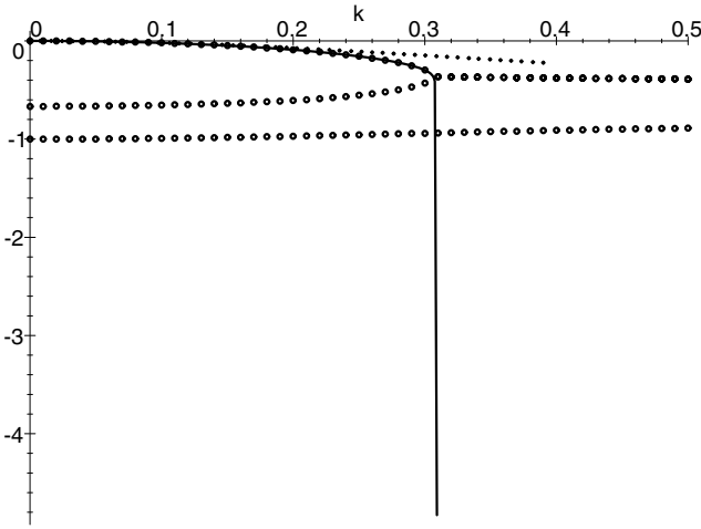
Fig. 9 Solutions to the Eq. (123). Circles: Numerical solutions. Dots: The first Newton iteration. Solid: The 4th Newton iteration
