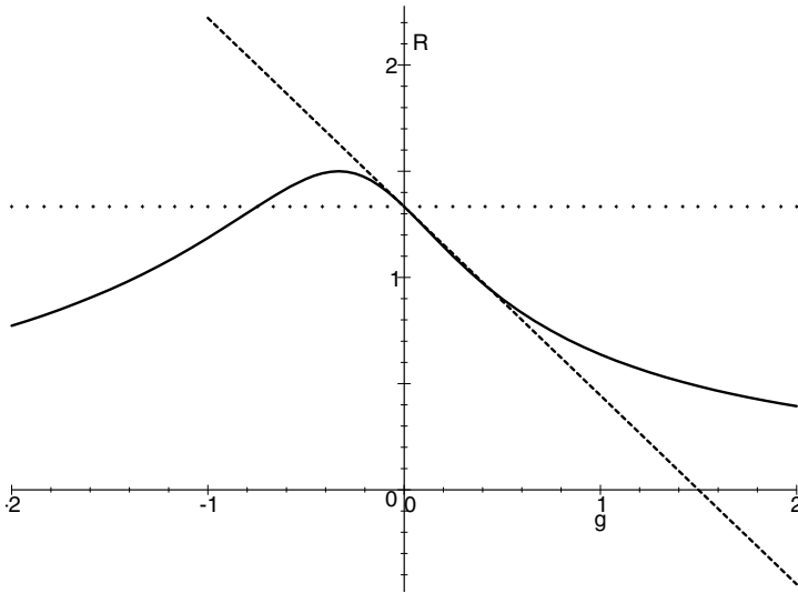
Fig. 10 Viscosity factor R(g) for Maxwell molecules. Solid: exact solution. Dash: the Burnett approximation. Dots: the Navier-Stokes approximation
