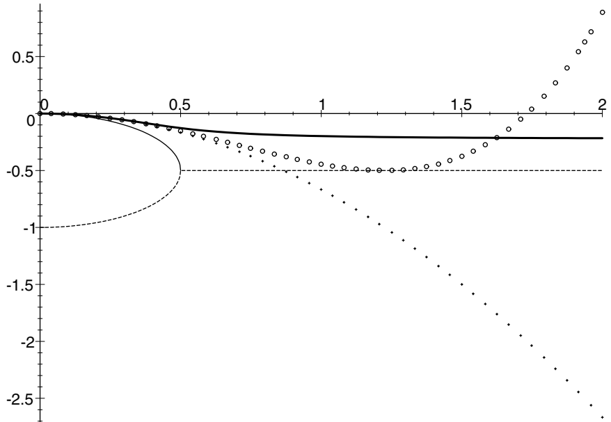
Fig. 3 Attenuation rates for the 3D10M Grad system. Bold: The acoustic branch, exact summation. Dots: The acoustic branch, Navier–Stokes approximation. Circles: The acoustic branch, super-Burnett approximation. Solid: The diffusion branch, exact summation. Dash: The critical mode of the 3D10M Grad system
