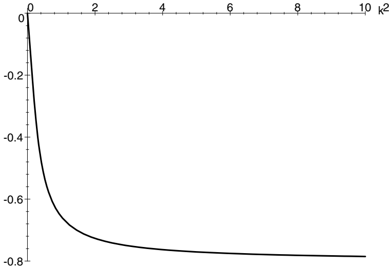
Fig. 1 Real-valued root of Eq. (33) as a function of k^2
