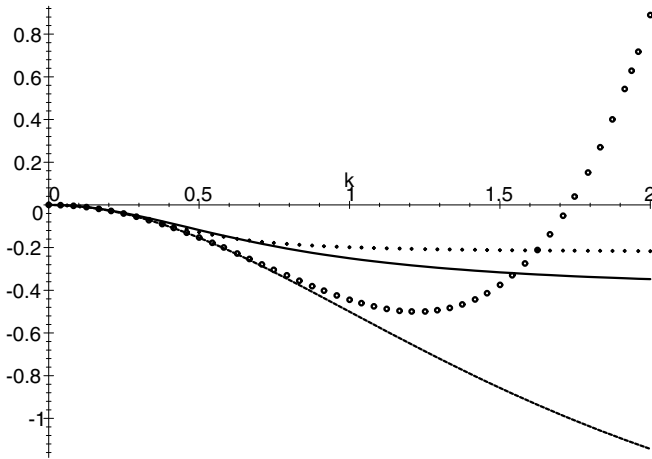
Fig. 4 Attenuation rates for the partial summation. Solid: The regularized Burnett approximation. Dash: The regularized super-Burnett approximation. Circles: The super-Burnett approximation. Dots: The exact summation
