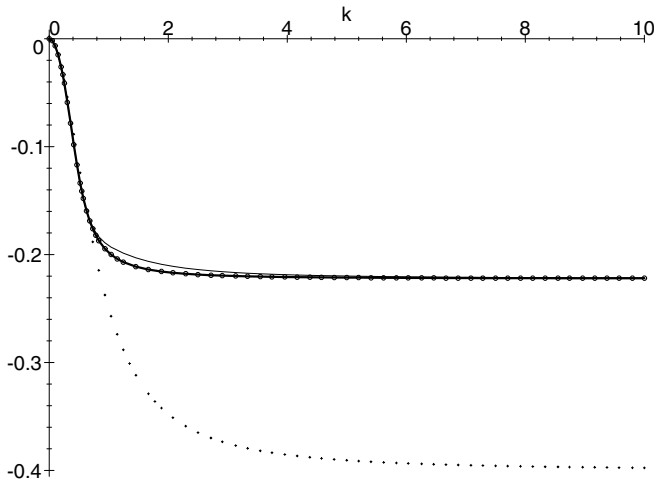
Fig. 6 Attenuation rates with the regularized Burnett approximation as the initial condition for the Newton method. Dots: The regularized Burnett approximation, or the first Newton iteration with the Euler initial condition (see text). Solid: The first and the second Newton iterations with the regularized Burnett approximation as the initial condition. Circles: The exact solution to the invariance equation
