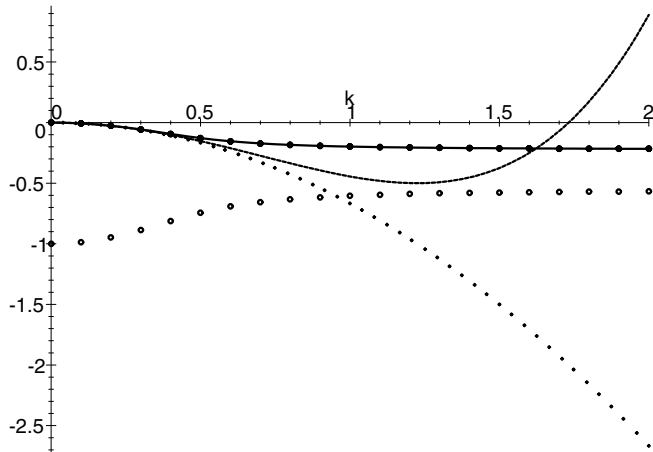
Fig. 2 Attenuation rates for the 1D10M Grad system. Solid: Exact summation of the Chapman–Enskog Expansion. Dots: The Navier–Stokes approximation. Dash: The super–Burnett approximation. Circles: Hydrodynamic and non-hydrodynamic modes of the 1D10M Grad system
