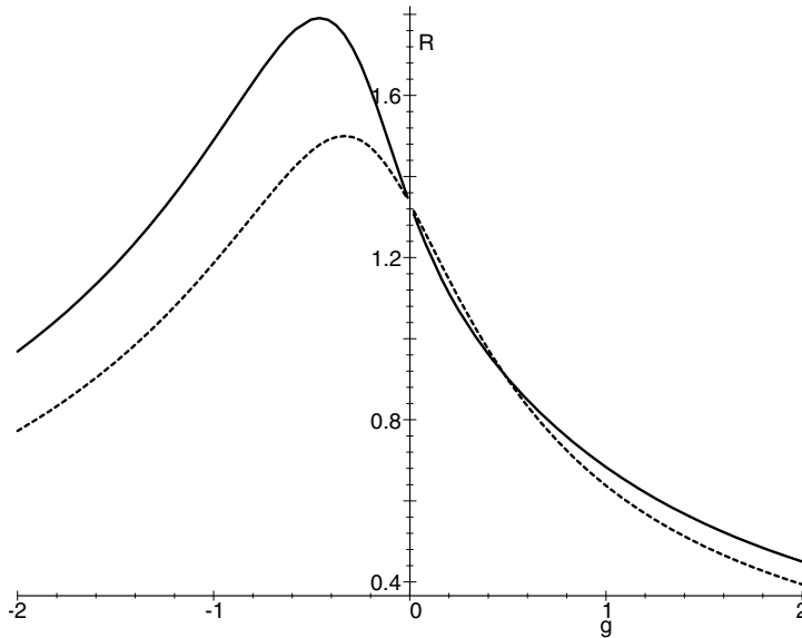
Fig. 11 Viscosity factor R(g) for hard spheres. Solid: the first approximation. Dash: exact solution for Maxwell molecules
