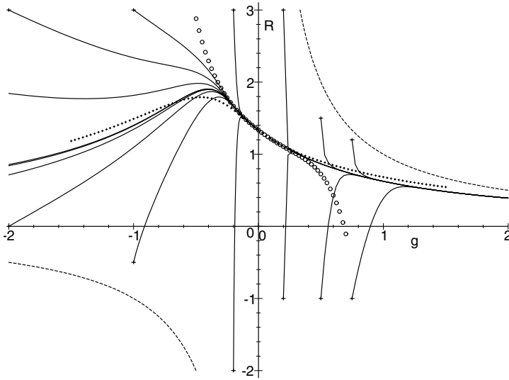
Fig. 12 Viscosity factor as an attractor. Solid lines: numerical integration with various initial points (crosses). Two poorly resolved lines correspond to the initial conditions (-100, 0) and (-100, 3) . Circles: Taylor expansion to the 5th order. Dots: the analytical approximation of (179). Dash: boundaries of the basin of attraction
