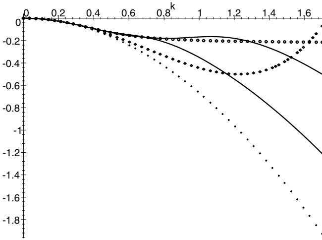
Fig. 5 Attenuation rates for the Newton method with the Navier–Stokes approximation as the initial condition. Dots: The Navier–Stokes approximation. Solid: The first and the second iterations of the invariance equation. Circles: The exact solution to the invariance equation. Diamond: The super-Burnett approximation
